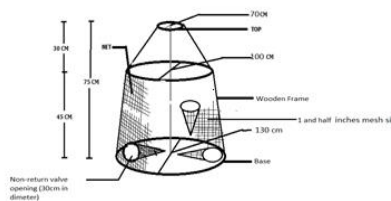
Fig:2 Sketch of a Traditional Malian Trap
