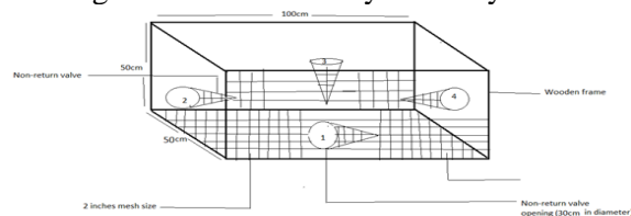
Fig 4: Sketch of Modified Rectangular Malian Trap
